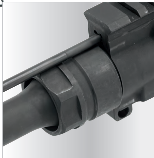
Steel Barrel Nut Compatible with Bull Barrels up to \text{Ø}1.05 " and Requires Little to No Timing
